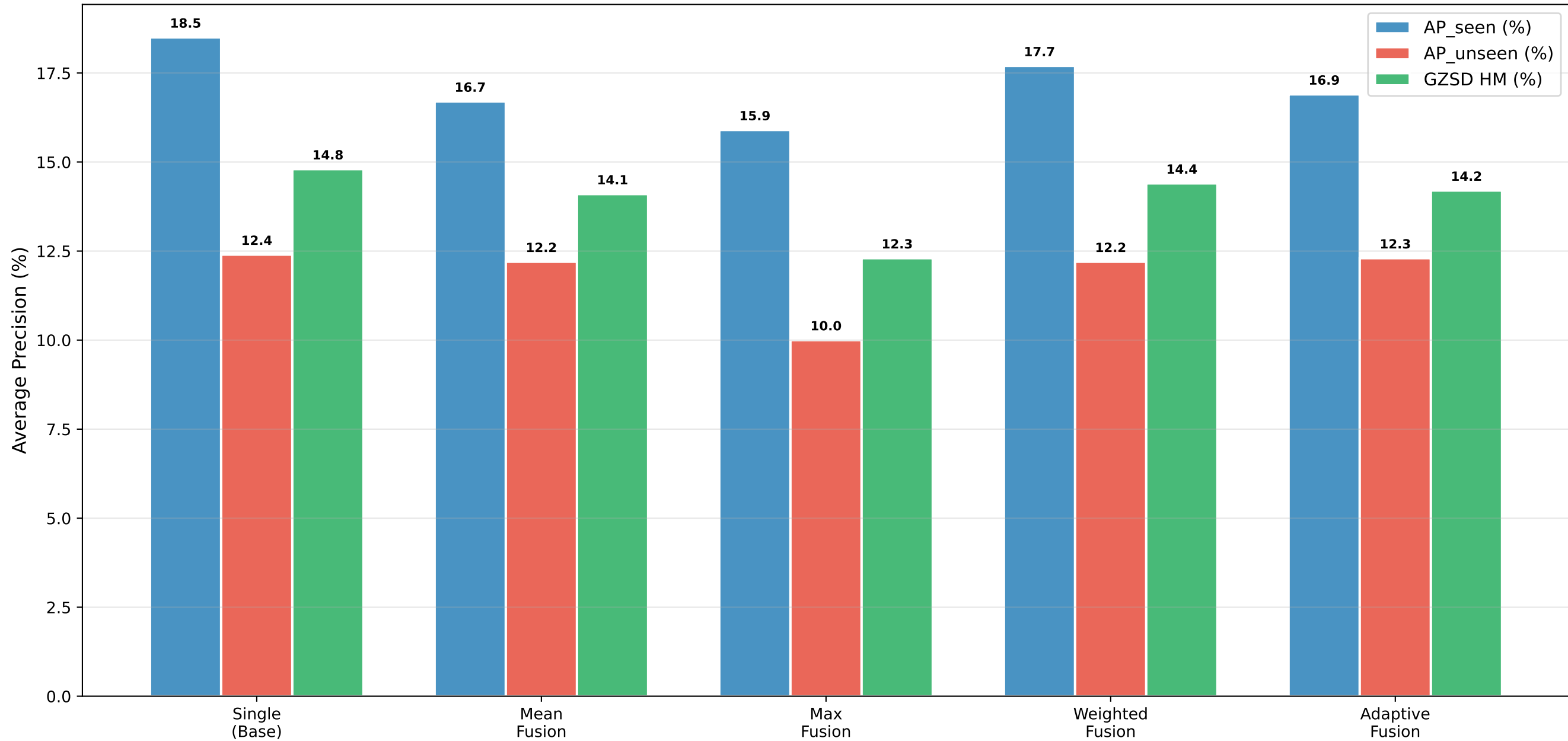
Fusion Strategy Comparison: AP_seen, AP_unseen, GZSD HM
